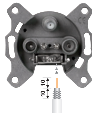
Contactdoos coax
